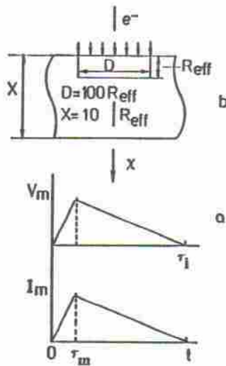
Fig. 1: Oscillograms of current and tension voltage of electronic beam (a) and the irradiate scheme (b)
