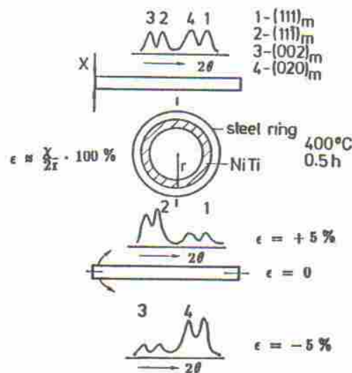
Fig. 2: Scheme of the deformation and diffractogram fragments for started and deformed state of NiTi-specimens
